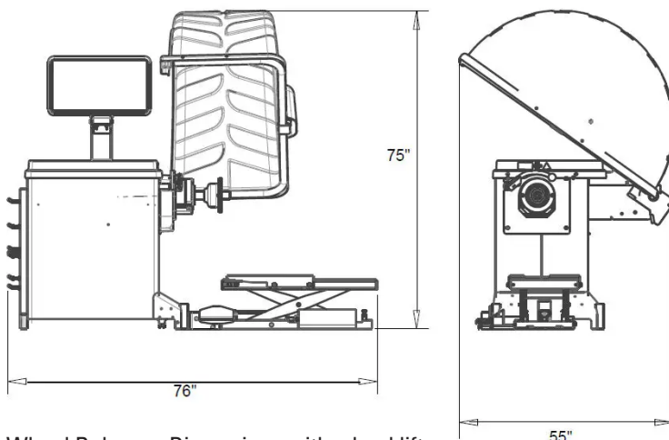
Wheel Balancer Dimensions with wheel lift
